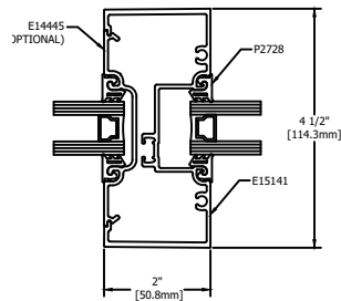
6 VERTICAL STANDARD
