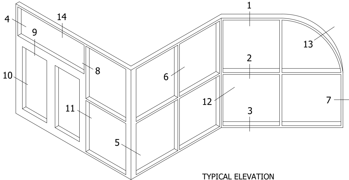
TYPICAL ELEVATION
