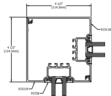
12 CORNER STANDARD
