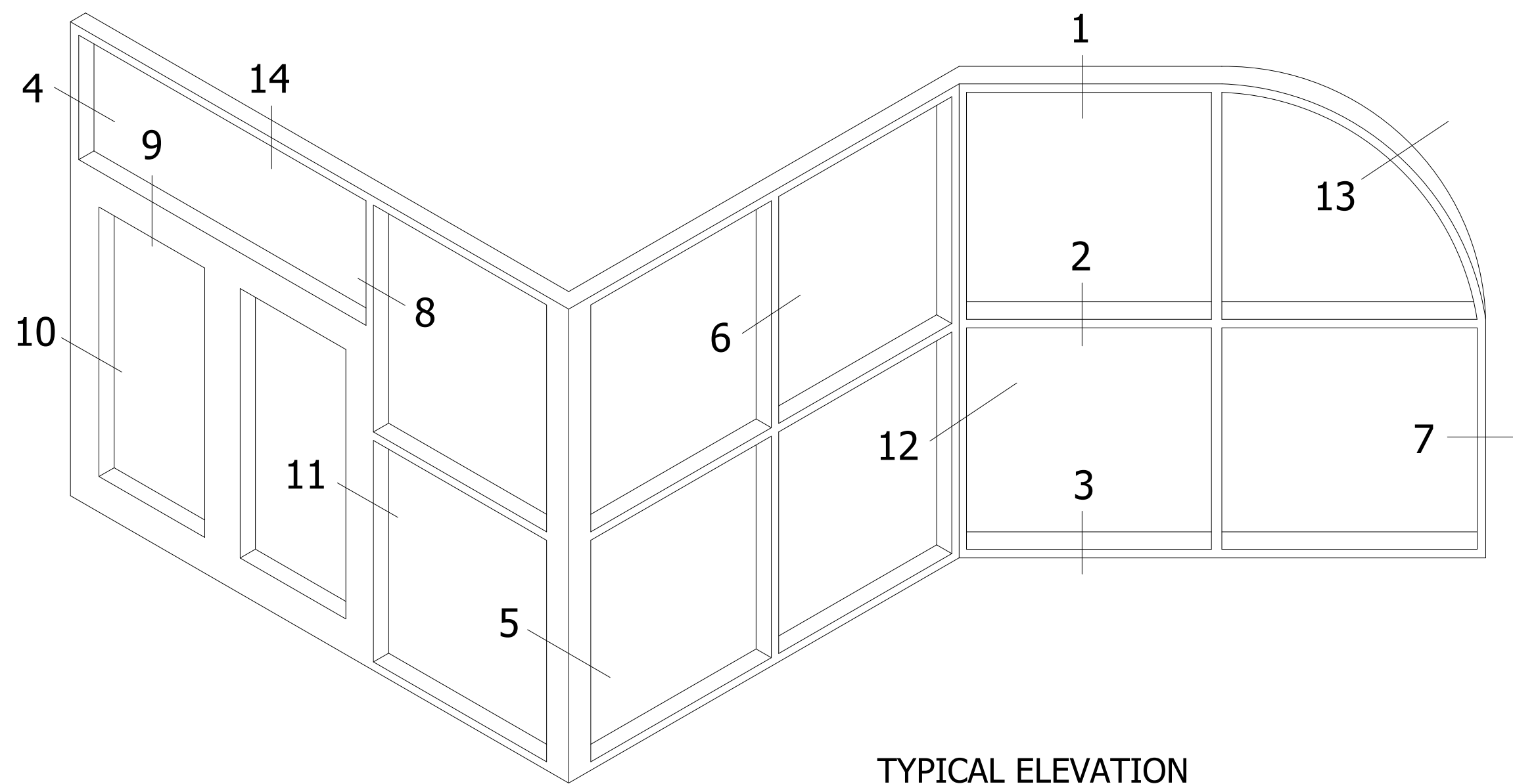
TYPICAL ELEVATION
