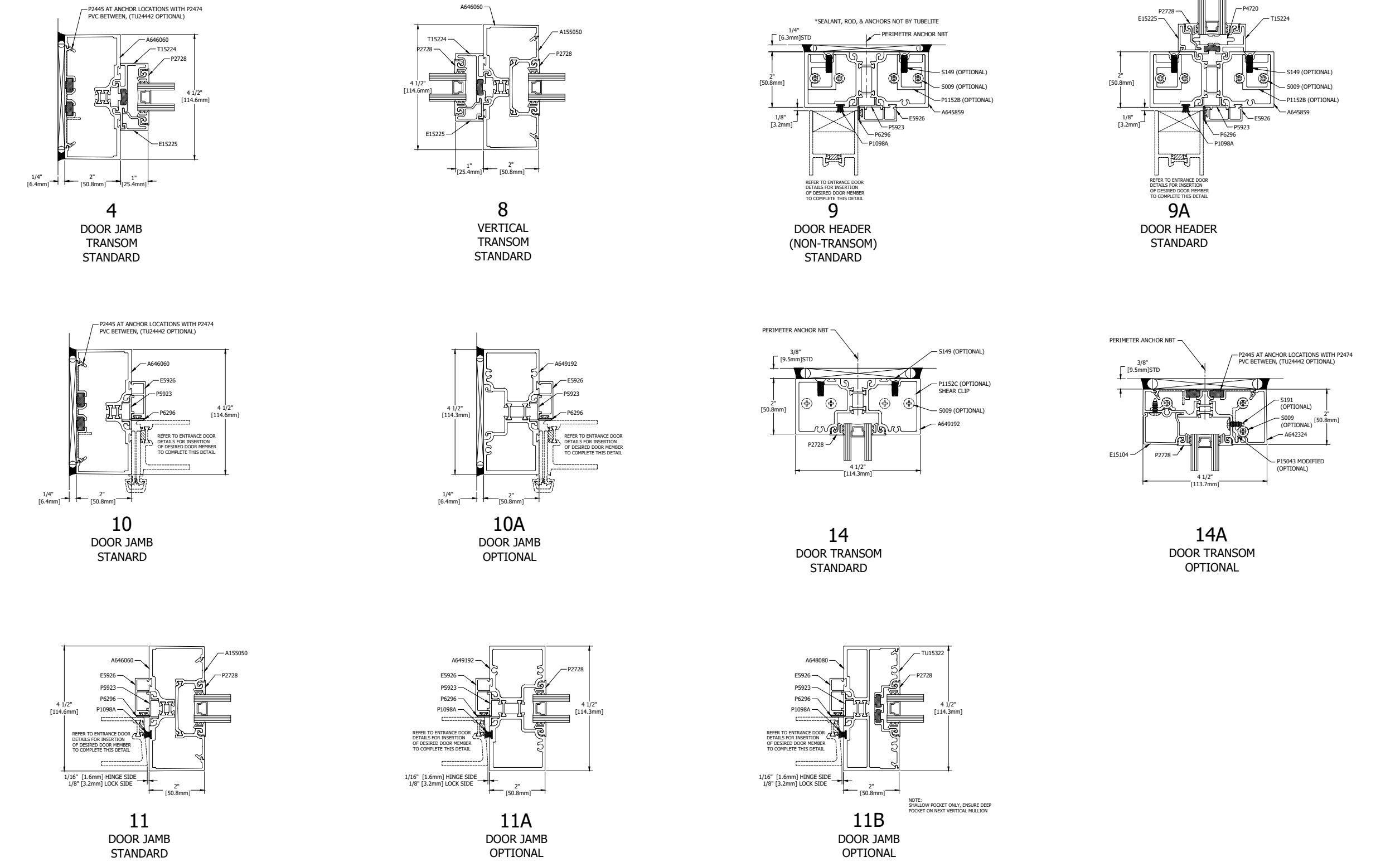
THERMAL DOOR DETAILS OHCC OR OTHER SPECIFIC CONDITIONS MAY REQUIRE NON-THERMAL DETAILS, REFER TO E14000 PERIMETER SHEET
