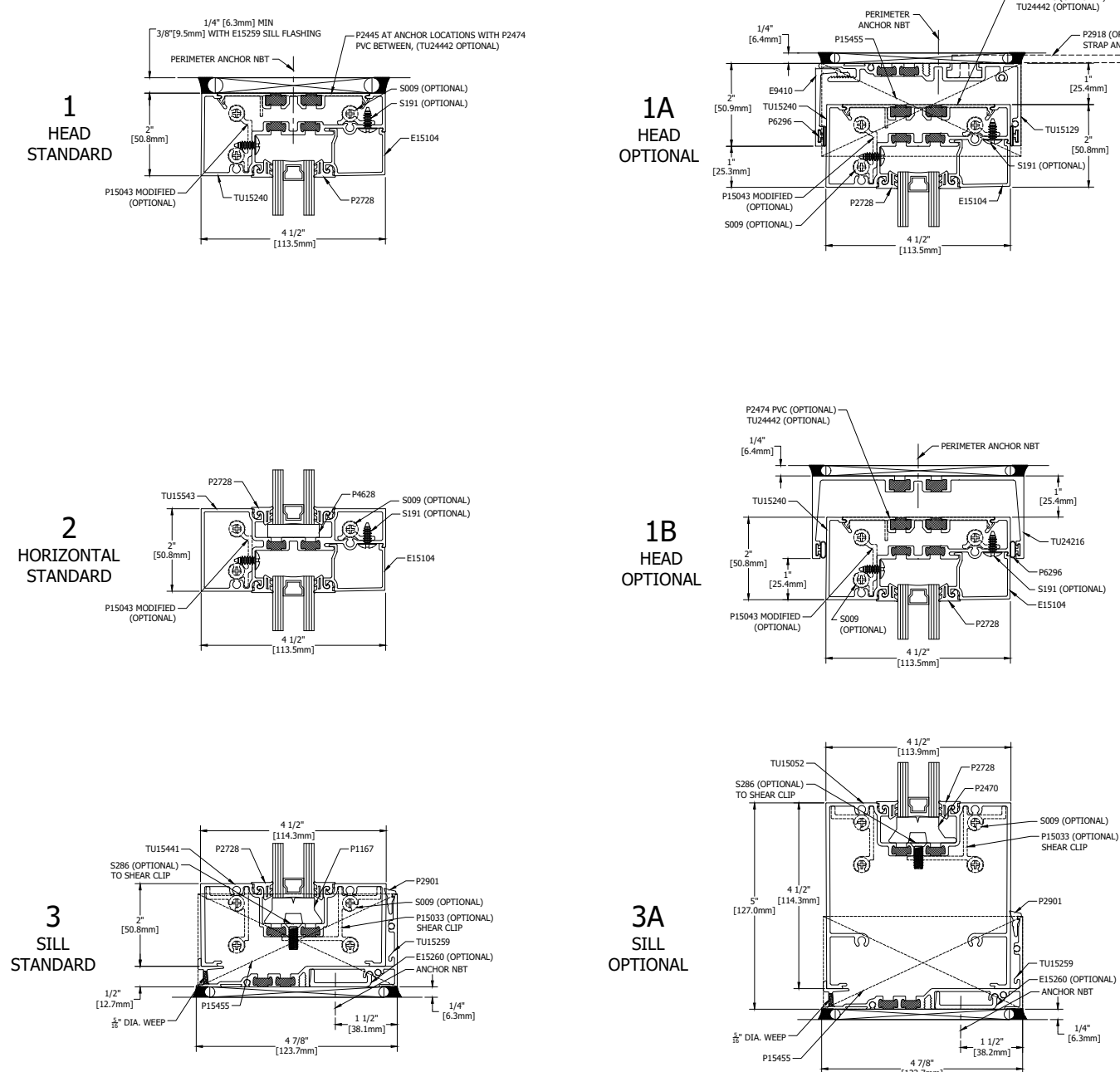
INSIDE GLAZED
