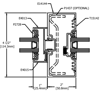
8 VERTICAL TRANSOM STANDARD
