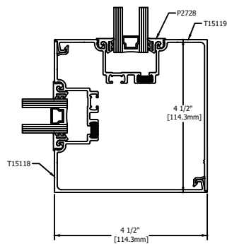
5 O.S. 90° CORNER STANDARD
