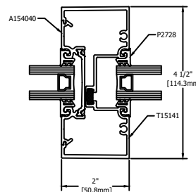
6 VERTICAL STANDARD
