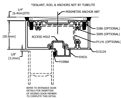
9 DOOR HEADER (NON-TRANSOM) STANDARD
