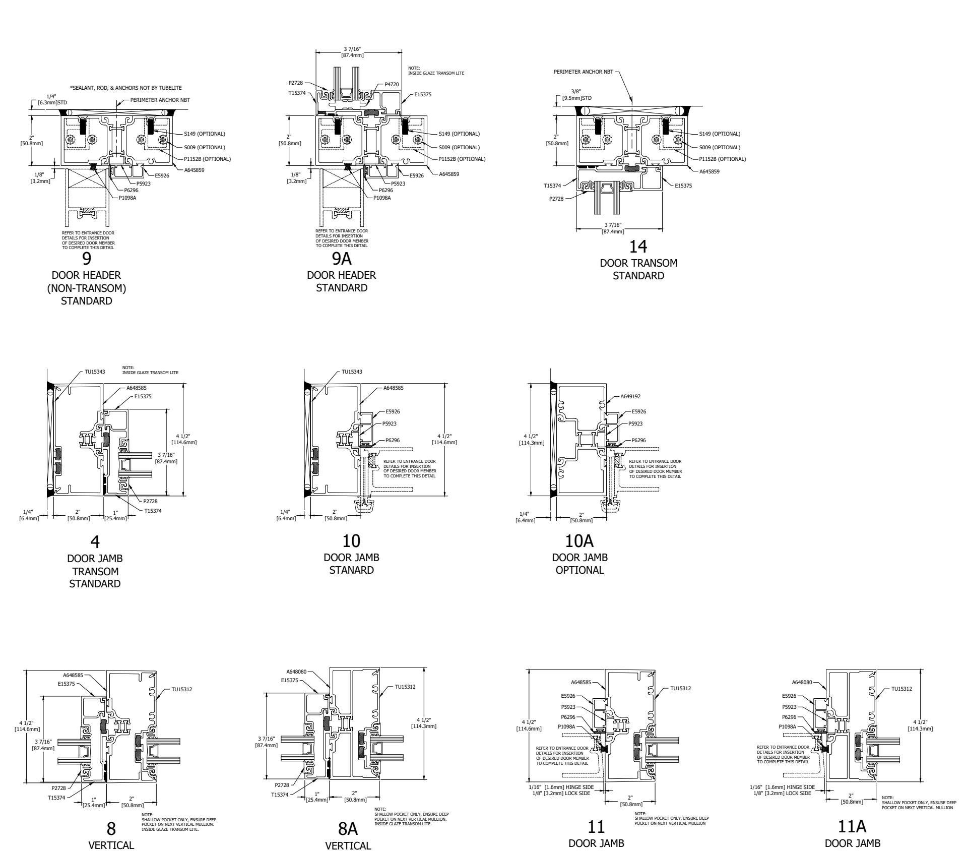
THERMAL DOOR DETAILS OHCC OR OTHER SPECIFIC CONDITIONS MAY REQUIRE NON-THERMAL DETAILS, REFER TO E14000 I/O PERIMETER SHEET
