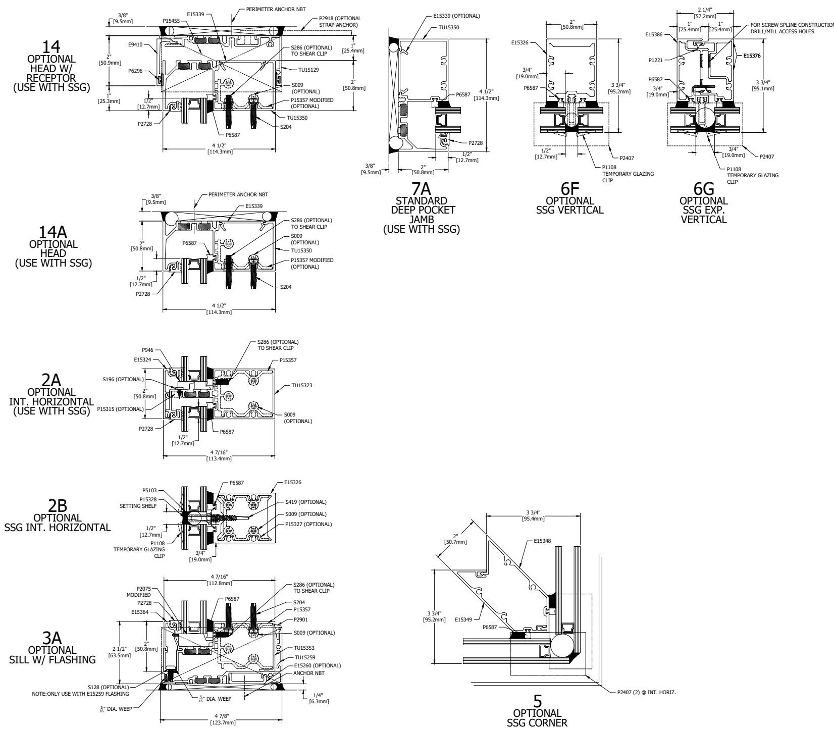
SSG OPTIONS (OUTSIDE GLAZE)
