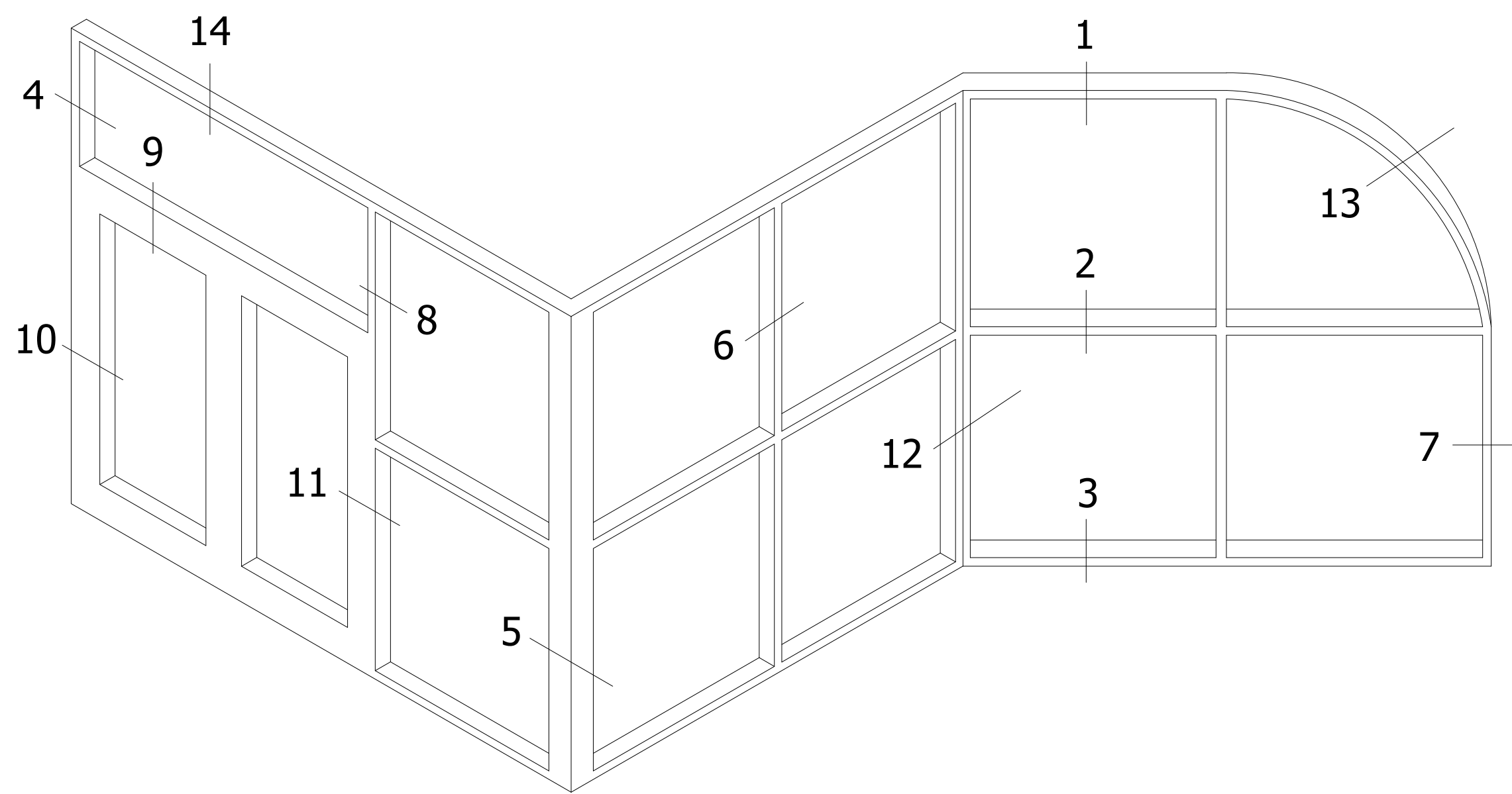
TYPICAL ELEVATION
